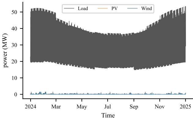
Network profiles — cigre_mv_pv_wind
